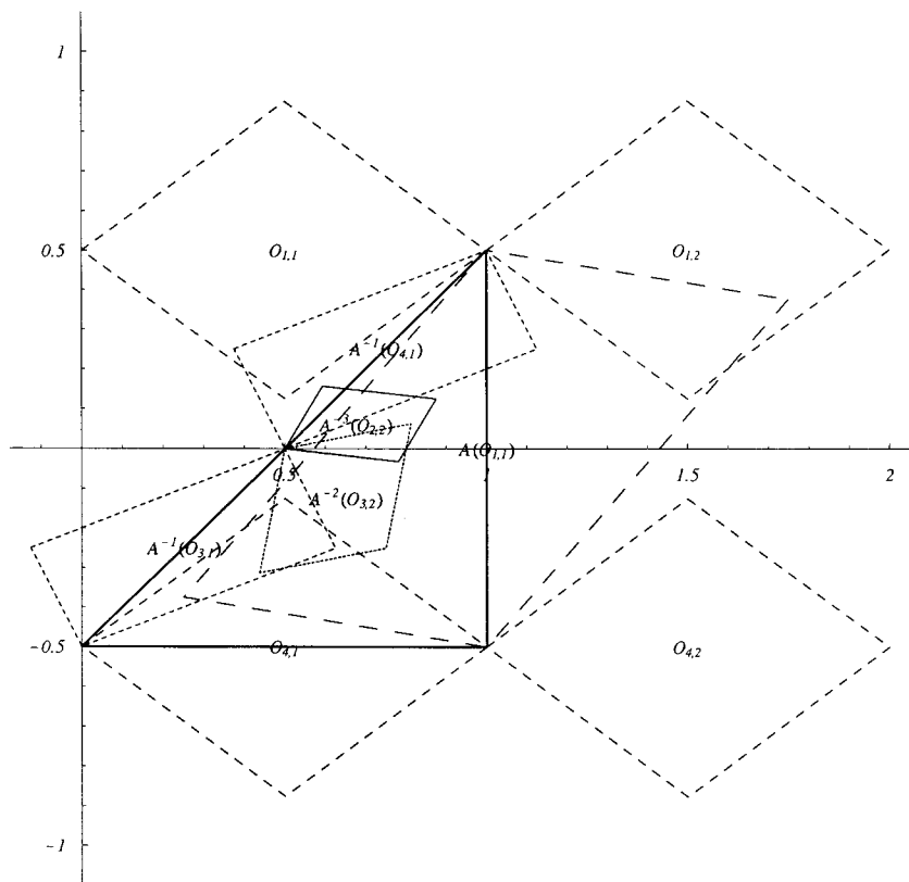
FIG. 2. Verification of Proposition 2.2.
