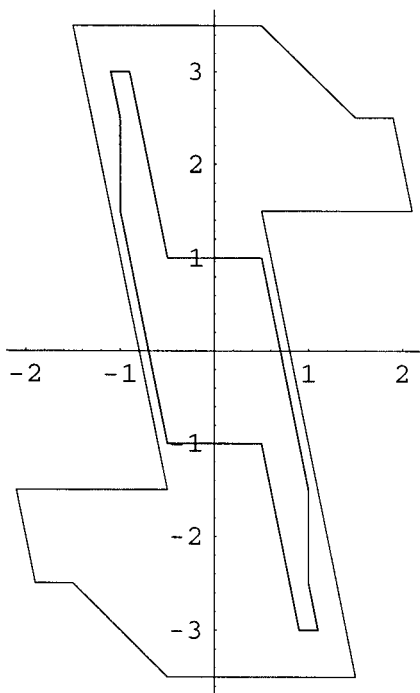
FIG. 5. Strict expansiveness for trace 0, \text{Det} \geq 4 .
