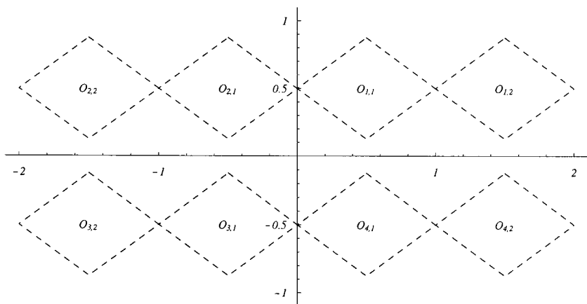
FIG. 1. Zero set of m_0 .
