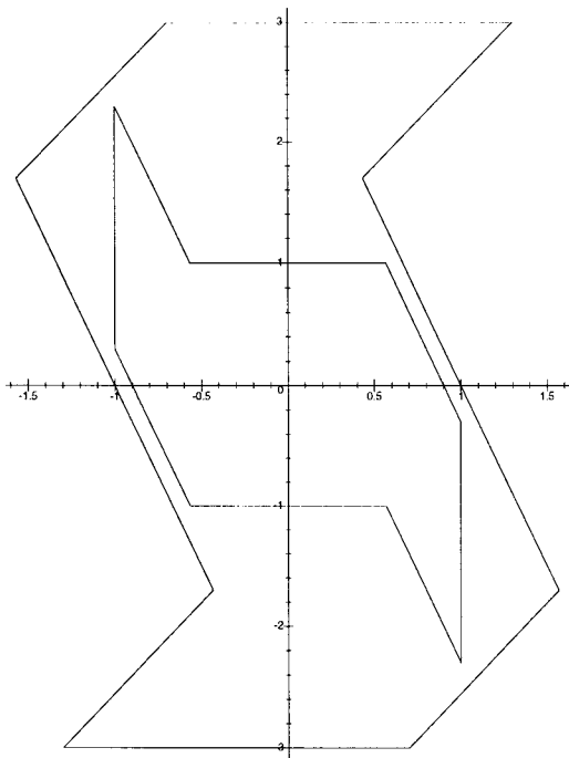
FIG. 4. Strict expansiveness for trace 1.
