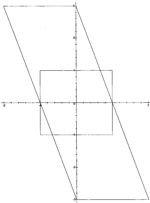
FIG. 3. First try for strict expansiveness.
